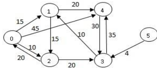
Output Graph:
