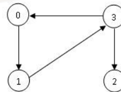
Input Graph:
