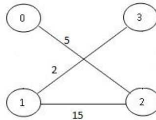
Output Graph:
